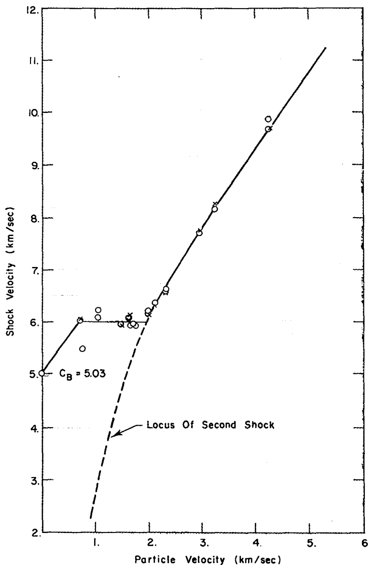
Fig. 8. Experimental Hugoniot data for lithia-boria glass compared with predictions of the SESAME EOS (solid and dashed curves). For particle velocities below .8 km/sec there is no phase transition and a single shock wave is stable. For particle velocities greater than 2 km/sec, the substance transforms to the high density phase and a single shock wave is stable. For intermediate velocities, calculations predict two shock waves. The leading wave corresponds to the low density phase and has U_p = .8 km/sec, U_s = 6 km/sec. The calculated locus of the second shock is shown by a dashed line; this wave has not been studied experimentally.
