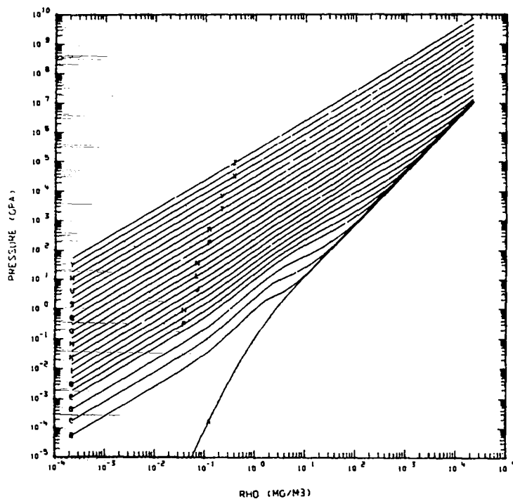
Fig. 13b. Ionic contribution to pressure-density isotherms of silicon dioxide over the temperature range 0.0-5.4 \times 10^8 K.
