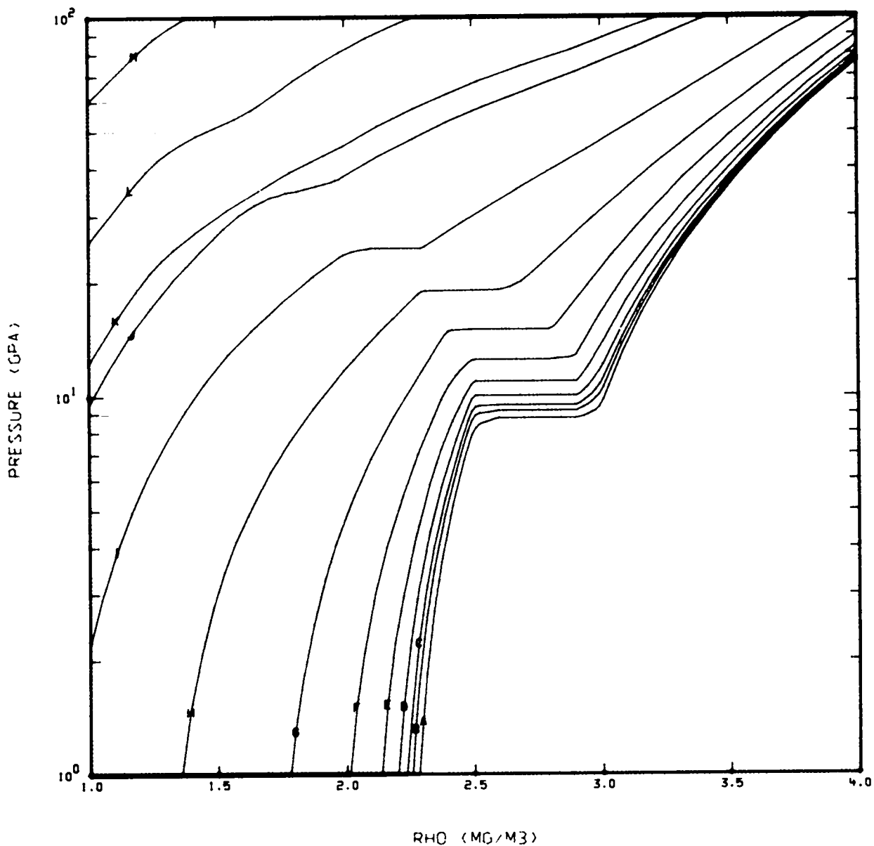
Fig. 9. Pressure-density isotherms for LiB glass in the region of phase transition.
