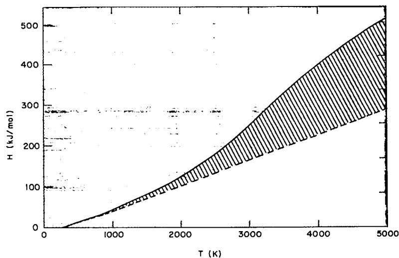
Fig. 15. \text{UO}_2 enthalpy ( H ) vs. temperature along liquid-vapor coexistence curve calculated with electronic excitations (solid curve) and without (dashed curve).
