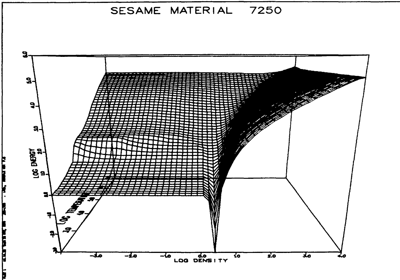
Fig. 1. EOS surface for lithia-boria glass, SESAME Material 7250, over densities 10^4 to 10^8 gm/cm 3 and temperatures 10^2 — 10^7 K.
