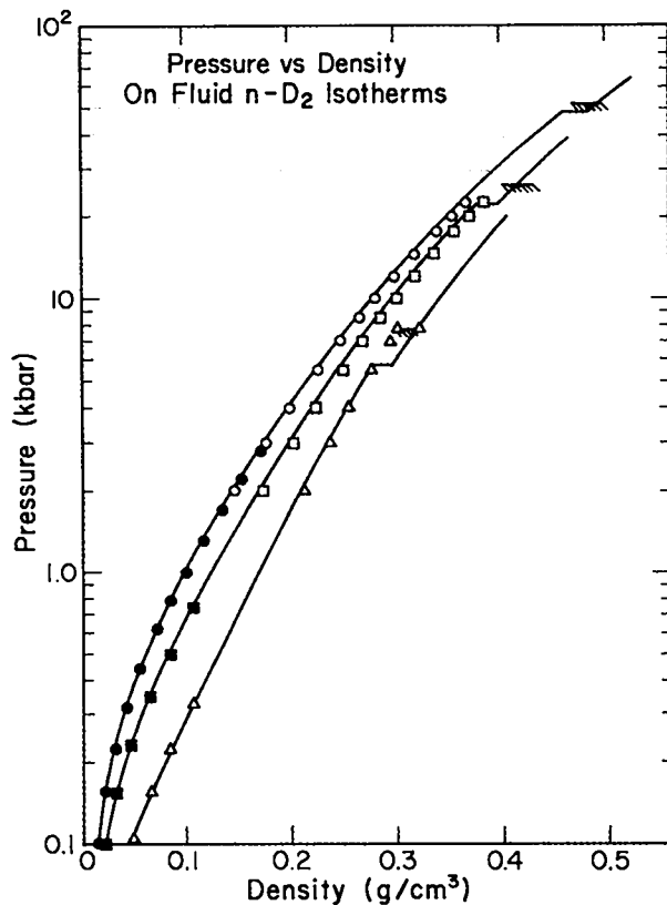
Fig. 11. Deuterium fluid isotherms. Experimental data 7 are compared with theoretical prediction (solid curves) for pressure vs. density.
