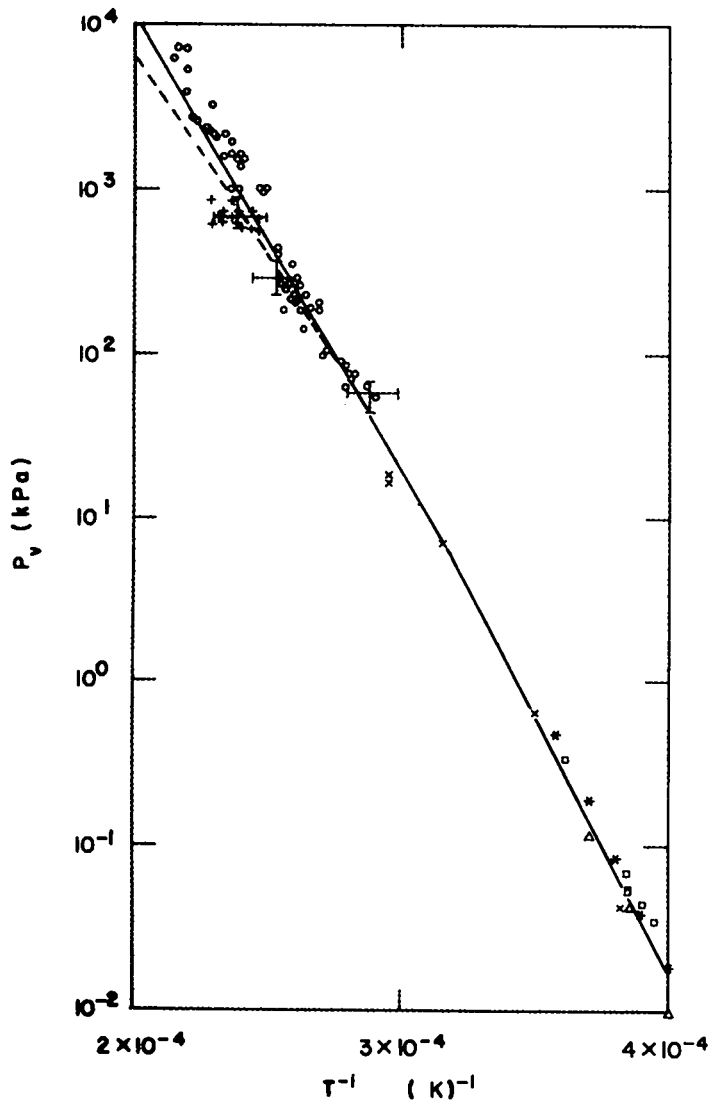
Fig. 16b. UO_2 vapor pressure for high temperatures. Calculated values (solid curve) are compared with experimental data points and IAEA standard (dashed curve).
