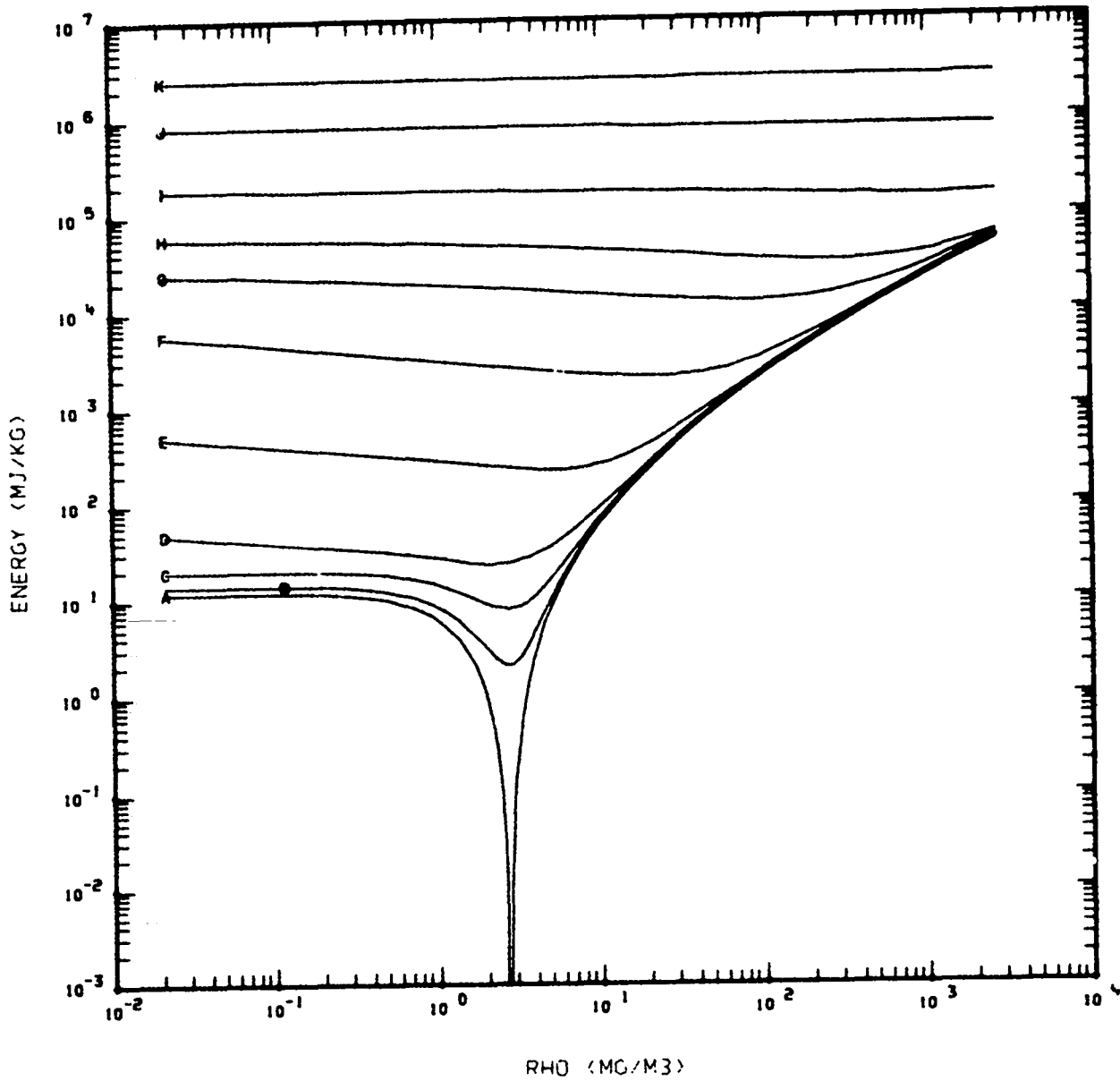
Fig. 6. Graph of aluminum energy-density-isotherms produced by the SES2D code.
