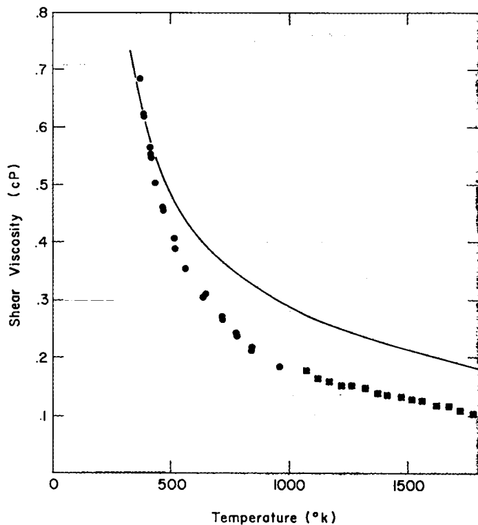
Fig. 19. (below left) Viscosity of liquid sodium. Calculated values (solid curve) are compared with experimental results. 16
