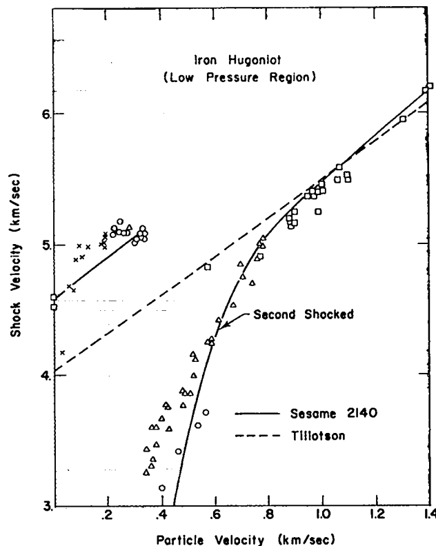
Fig. 2. Experimental data for the iron Hugoniot compared with predictions from the SESAME tables (solid line) and the Tillotson analytic EOS (dashed line).
