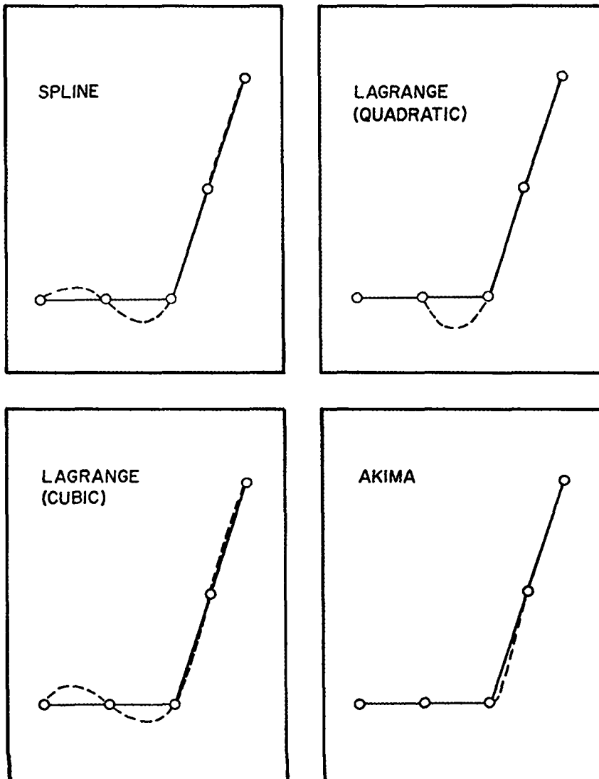
Fig. 3. Interpolation schemes applied to the intersection of two straight lines. The tabulated points are shown as circles.
