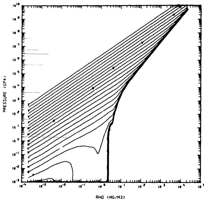
Fig. 13a. Ionic contribution to pressure-density isotherms of silicon dioxide over the temperature range 0.0-5.4 \times 10^8 K.
