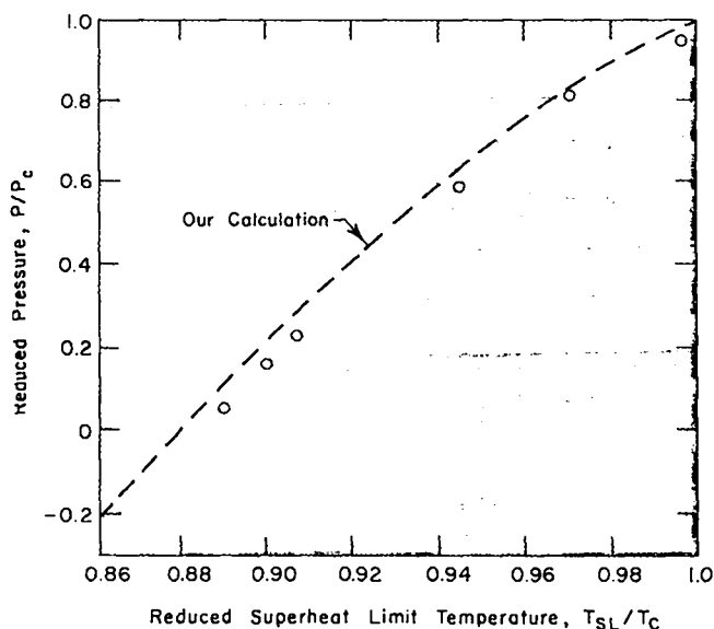
Fig. 20. Estimated limit of superheat temperatures from equation of state for dichlorodifluoromethane (R-12). Experimental values (circles) are reported by G. R. Moore, "Vaporization of Superheated Drops in Liquids," Ph.D. thesis, U. of Wisc., Madison 1956; AICh E. J. 5, 458 (1959).
