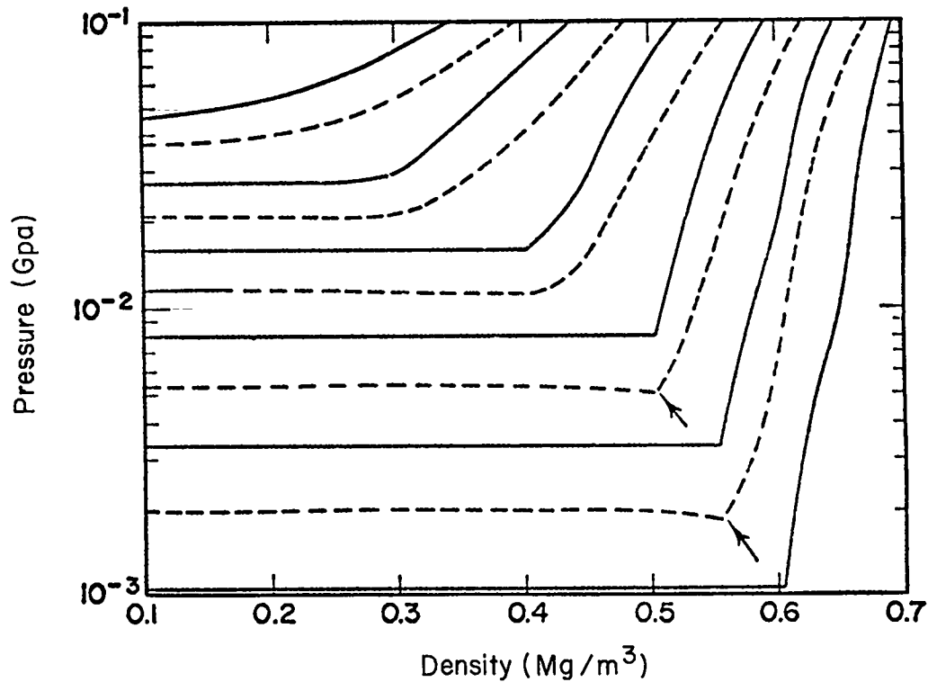
Fig. 4. Interpolated pressure-density-temperature surface.
