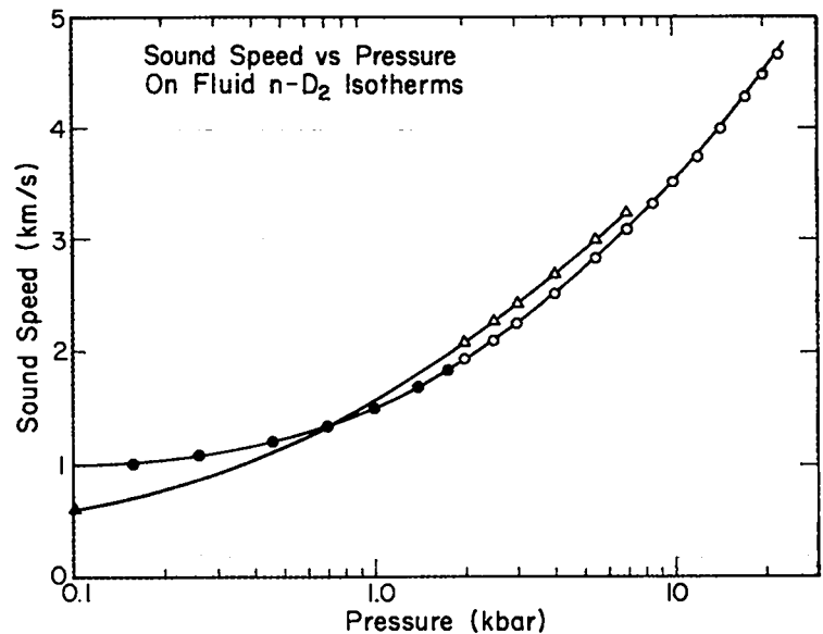
Fig. 12. Deuterium sound speed vs. pressure. Experimental data 7 are compared with theoretical prediction (solid curves).
