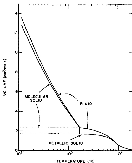
Fig. 10b. Specific volumes on the phase lines of deuterium (from Ref. 5).
