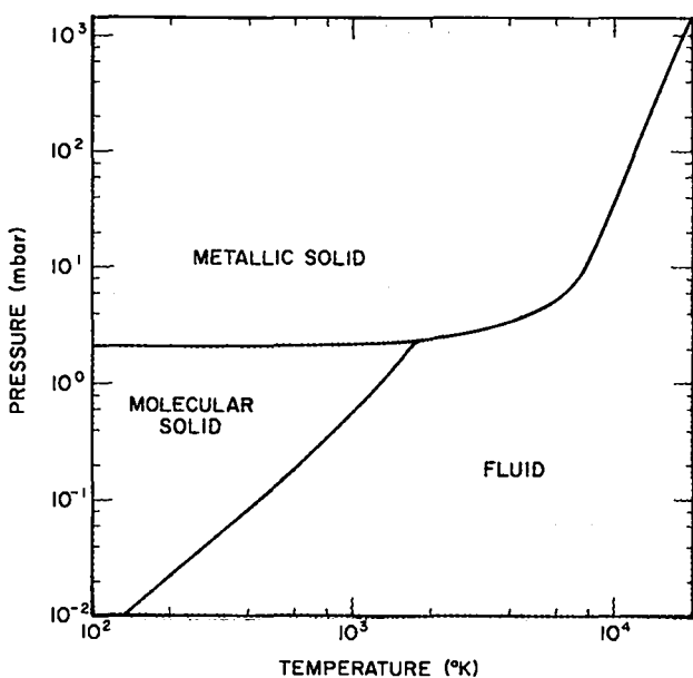
Fig. 10a. Phase diagram for deuterium (from Ref. 5).
