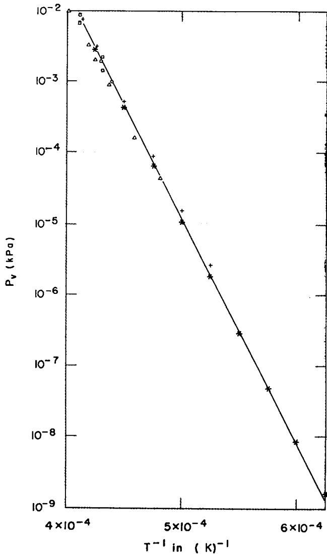
Fig. 16a. UO_2 vapor pressure for low temperatures. Calculated values (solid curve) are compared with experimental data points.
